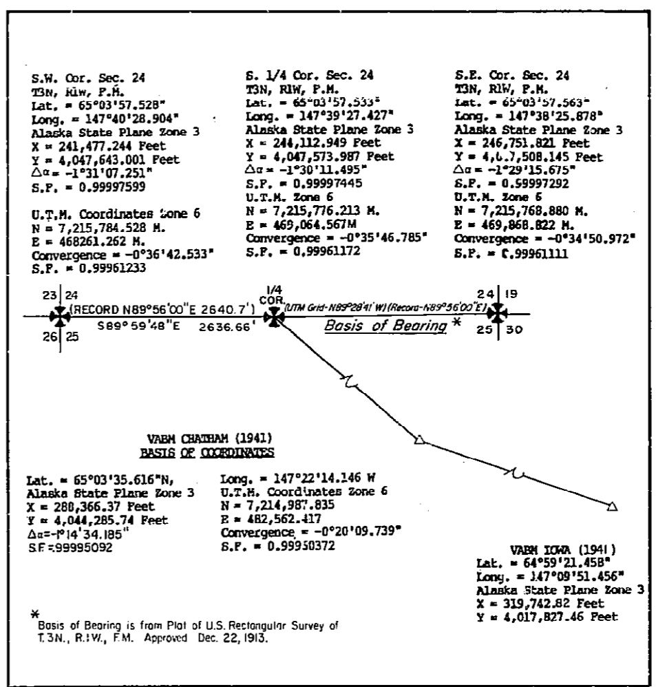
HORIZONTAL CONTROL DIAGRAM
